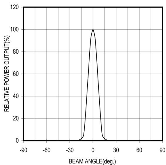
RADIATION PATTERN
