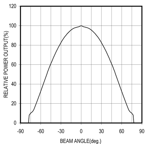
RADIATION PATTERN
