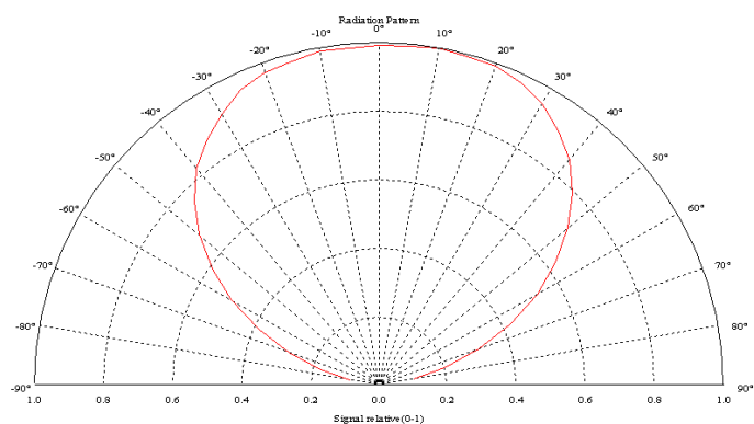
RADIATION PATTERN
