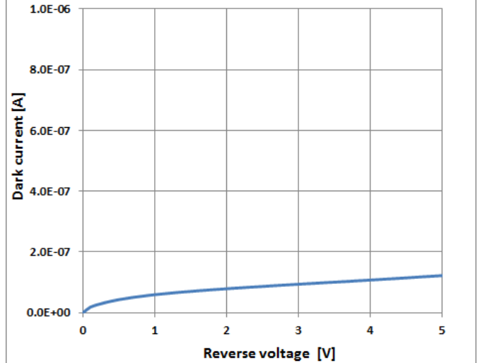
Dark current vs Reverse voltage
