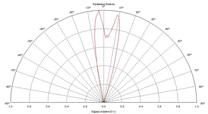
RADIATION PATTERN
