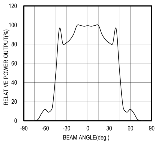
RADIATION PATTERN
