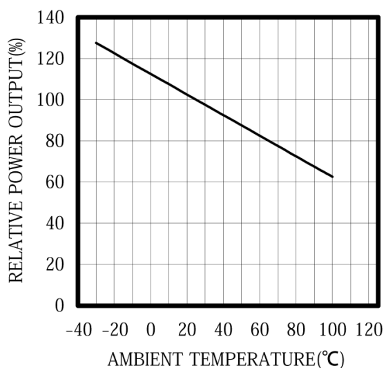
POWER OUTPUT vs TEMPERATURE IF=10mA
