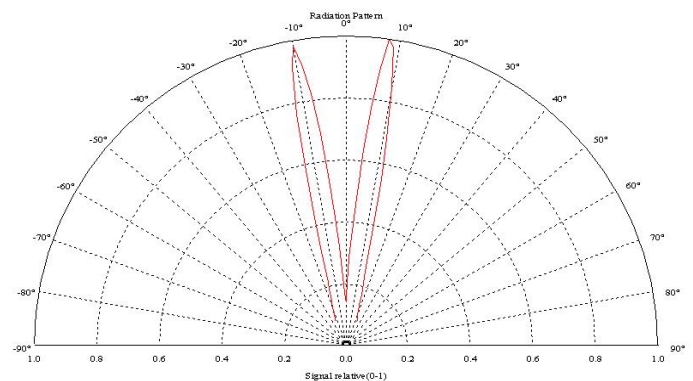
RADIATION PATTERN
