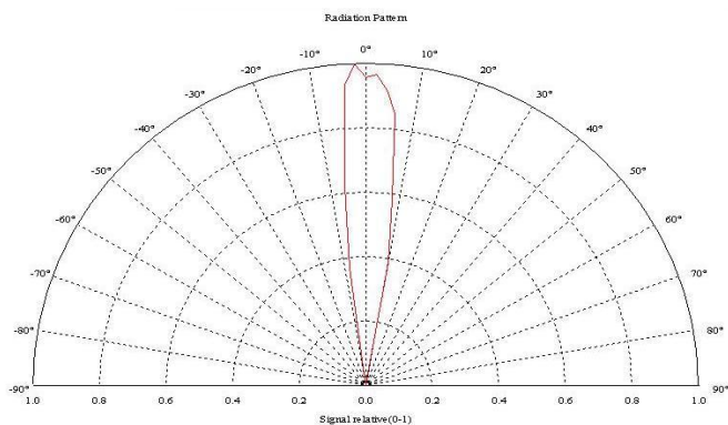
RADIATION PATTERN
