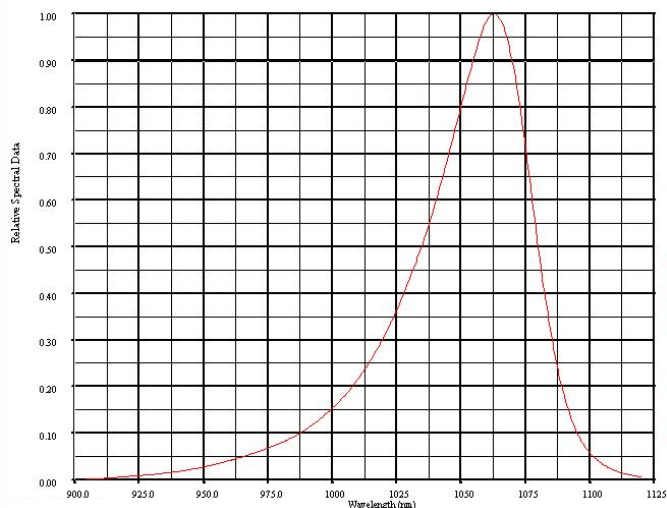
SPECTRAL OUTPUT
