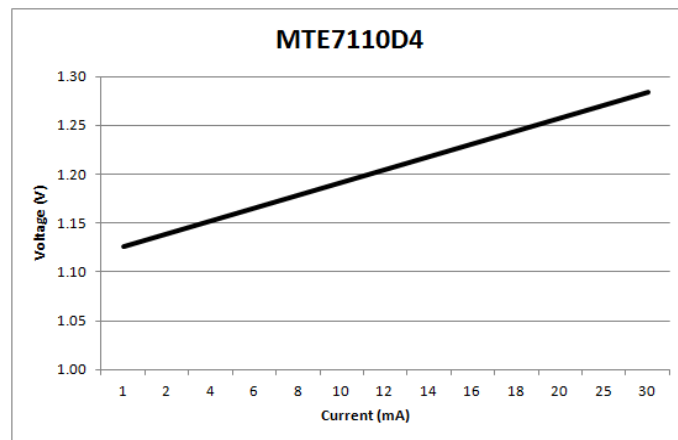
Forward V-I Characteristics
