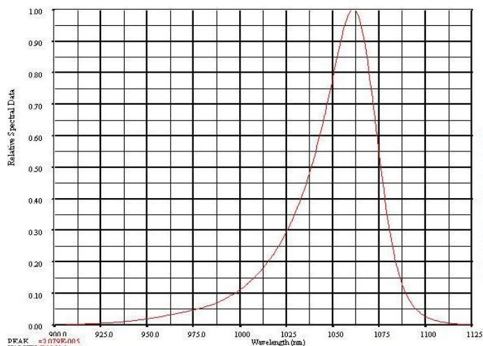
SPECTRAL OUTPUT
