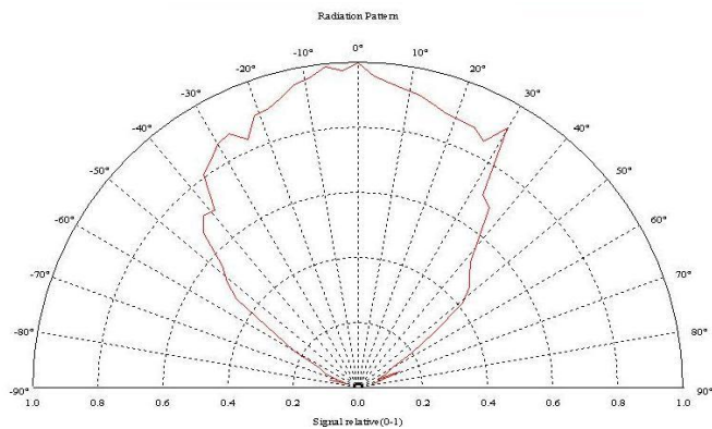
RADIATION PATTERN
