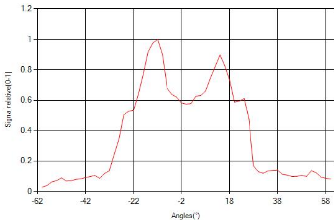
RADIATION DISTRIBUTION
