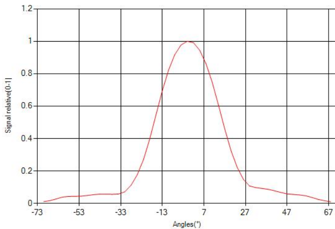
Radiation Distribution
