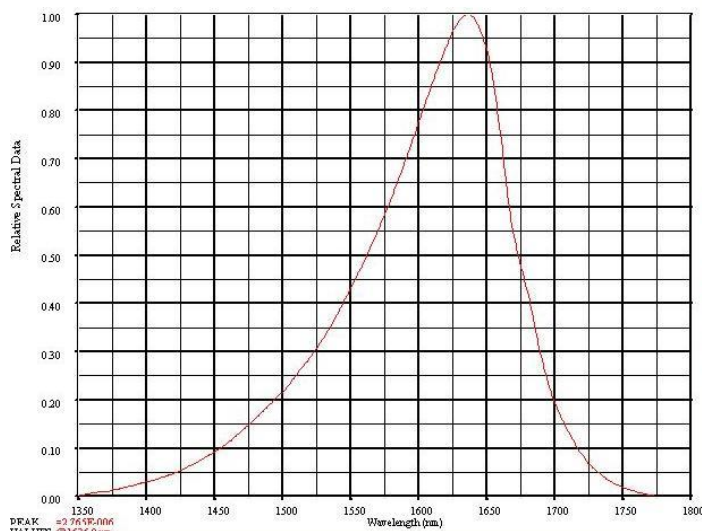
SPECTRAL OUTPUT
