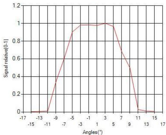
Radiation Distribution
