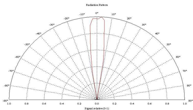
RADIATION PATTERN
