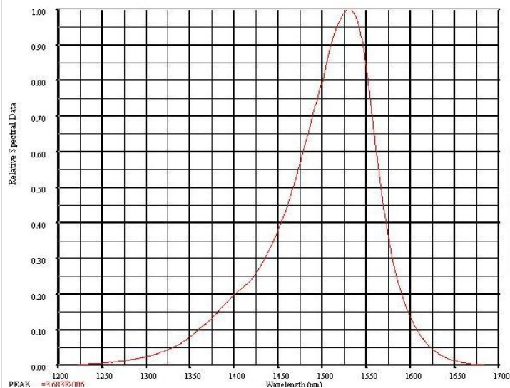
SPECTRAL OUTPUT
