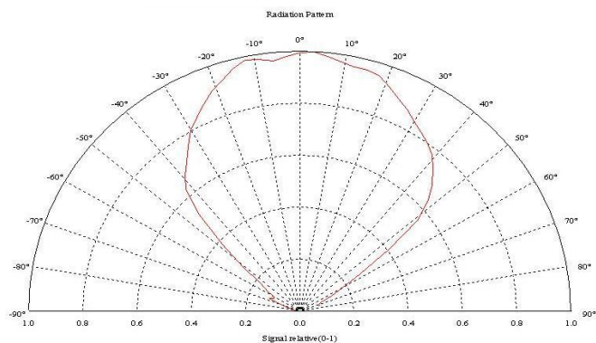
RADIATION PATTERN
