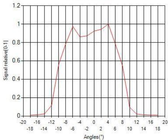
Radiation Distribution
