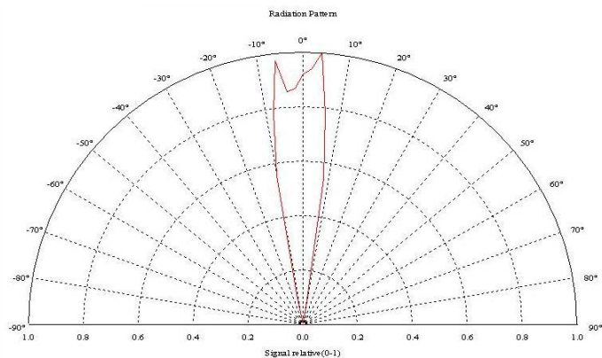
RADIATION PATTERN
