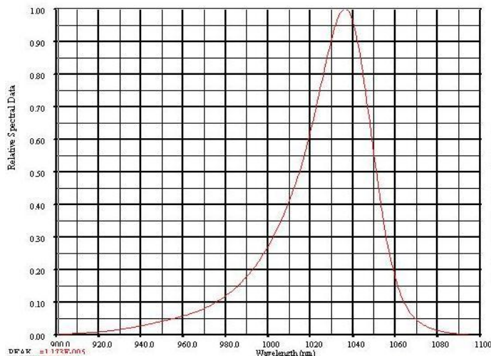
Spectral Output
