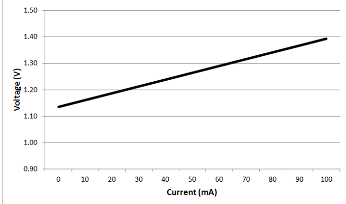
Forward I-V Characteristics
