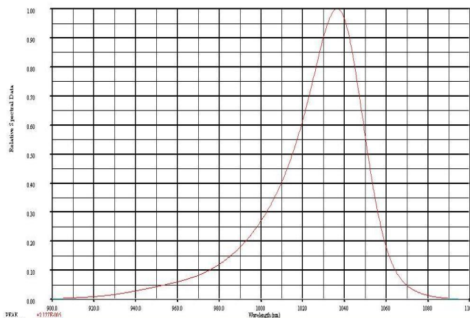
SPECTRAL OUTPUT
