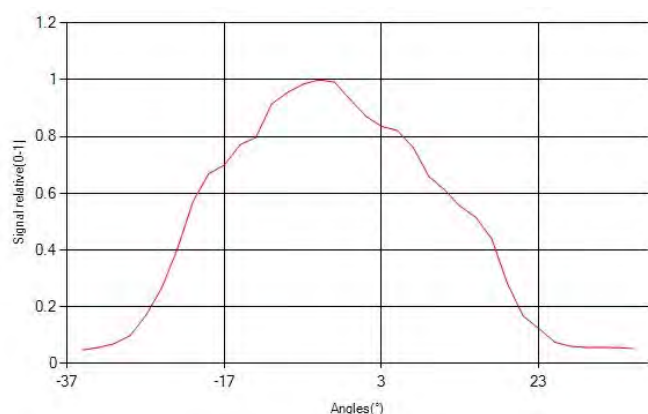
RADIATION DISTRIBUTION
