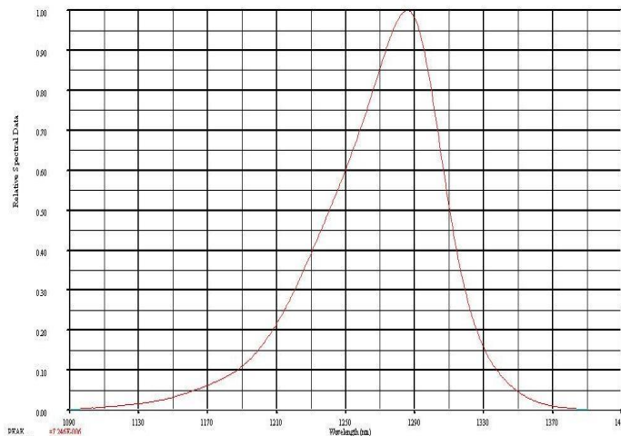
SPECTRAL OUTPUT
