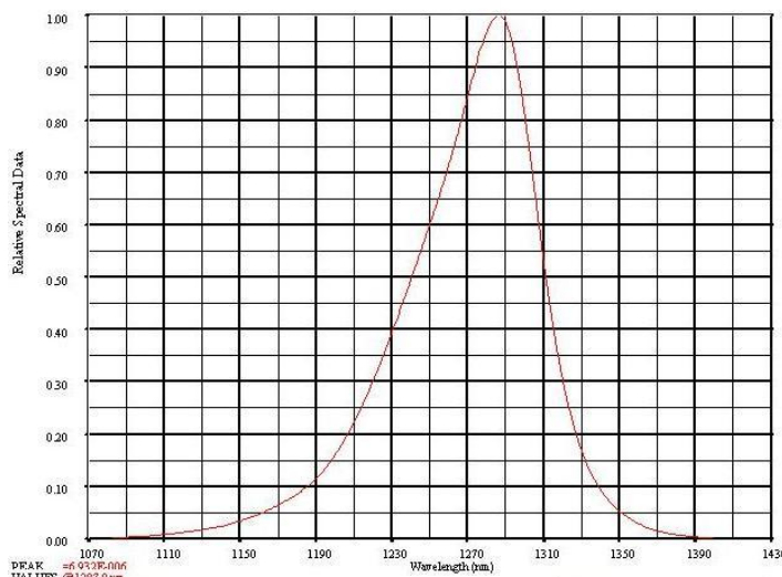
SPECTRAL OUTPUT
