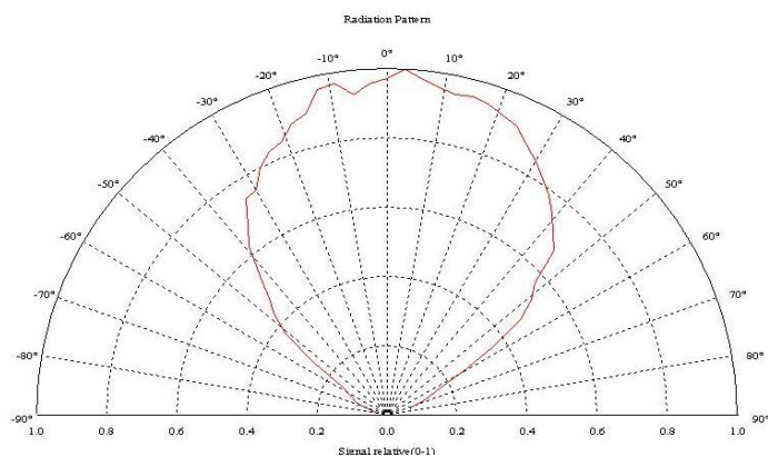
RADIATION PATTERN
