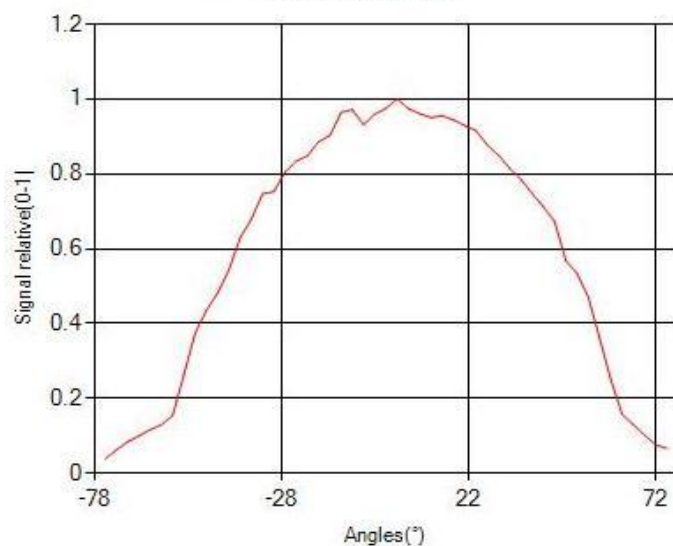
Radiation Distribution
