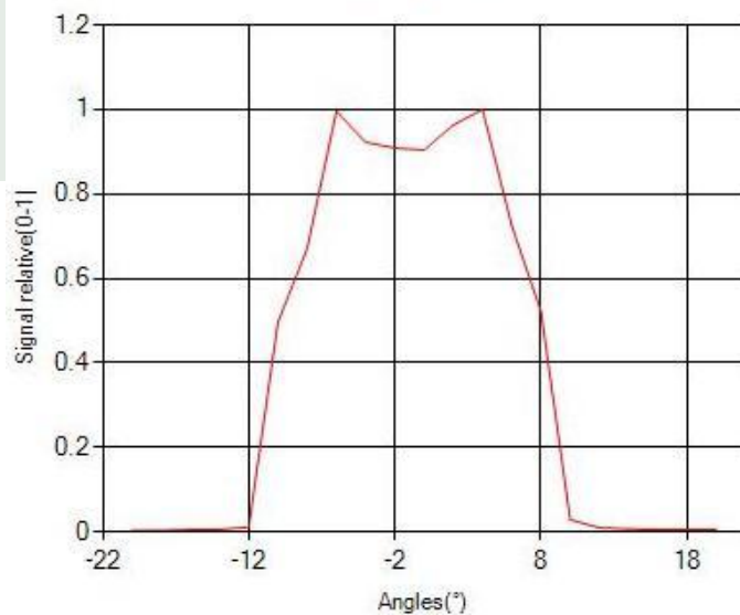
Radiation Distribution
