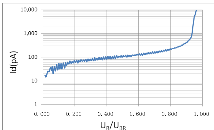
Fig 2 Dark Current
