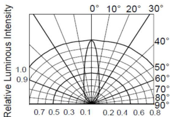
RADIATION DIAGRAM
