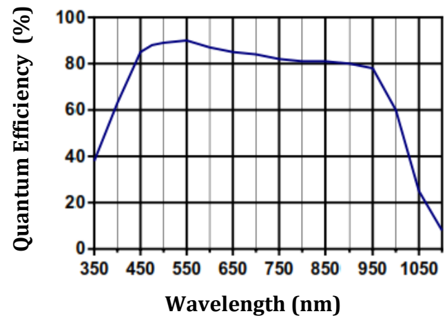
Quantum Efficiency (23 ^{\circ}C )
