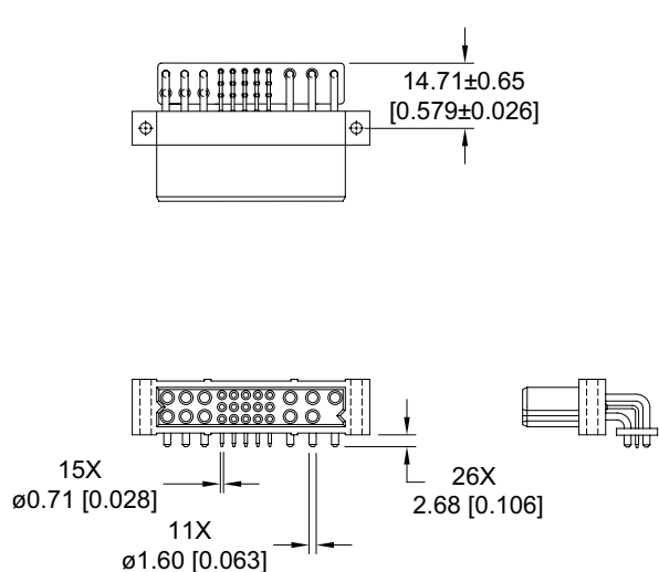
CONNECTOR DIMENSIONS
