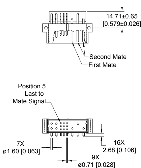
CONNECTOR DIMENSIONS
