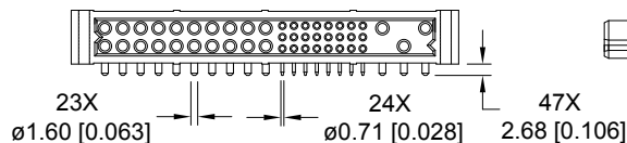
CONNECTOR DIMENSIONS
