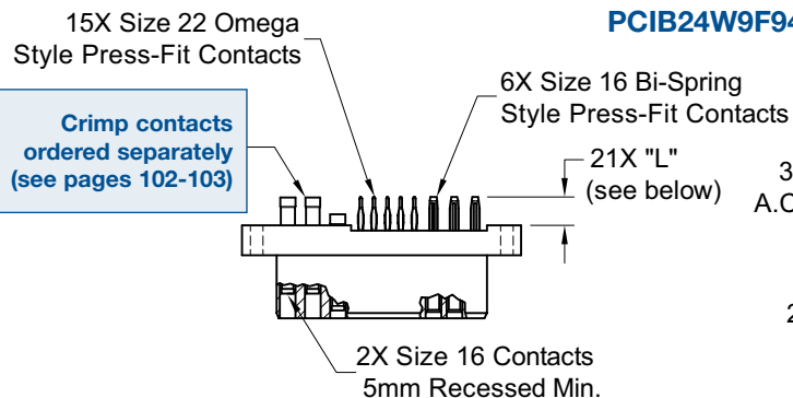
CONNECTOR DIMENSIONS
