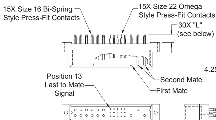
CONNECTOR DIMENSIONS
