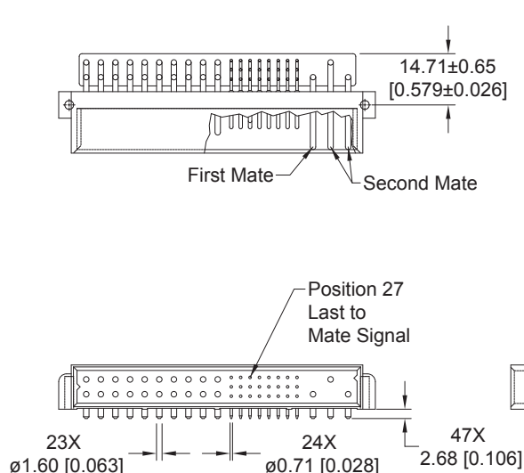
CONNECTOR DIMENSIONS
