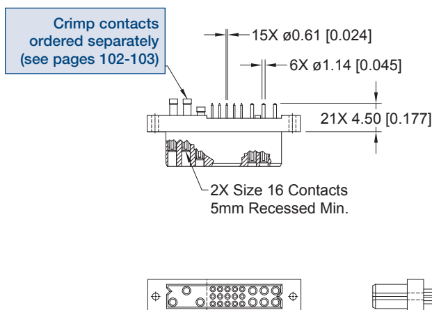
CONNECTOR DIMENSIONS
