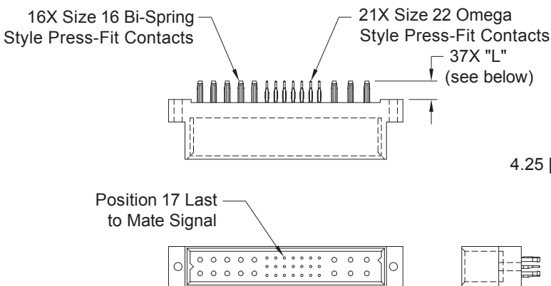
CONNECTOR DIMENSIONS
