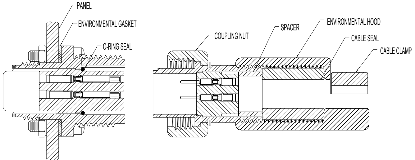
Fixed Female Flange Mounted Connector
