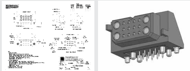
2-D Drawing
