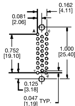
SGM 26 SGMC 26
