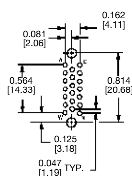
SGM 20 SGMC 20
