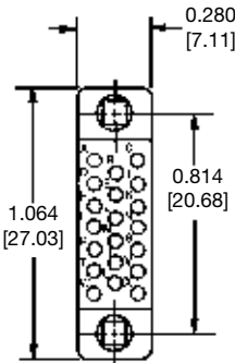
SGMC 20
