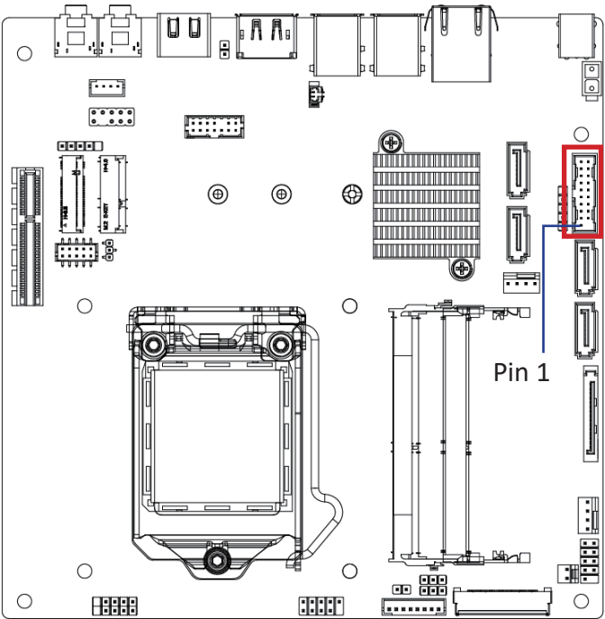
USB 3.0 Header
