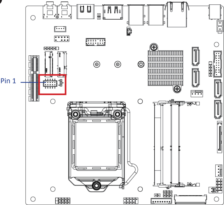
COM1 Connector
