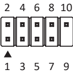
USB 2.0 Header
