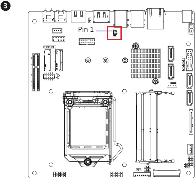
Battery Connector
