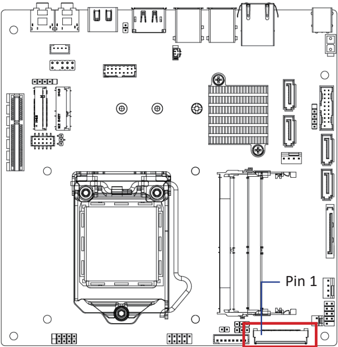
LVDS Connector
