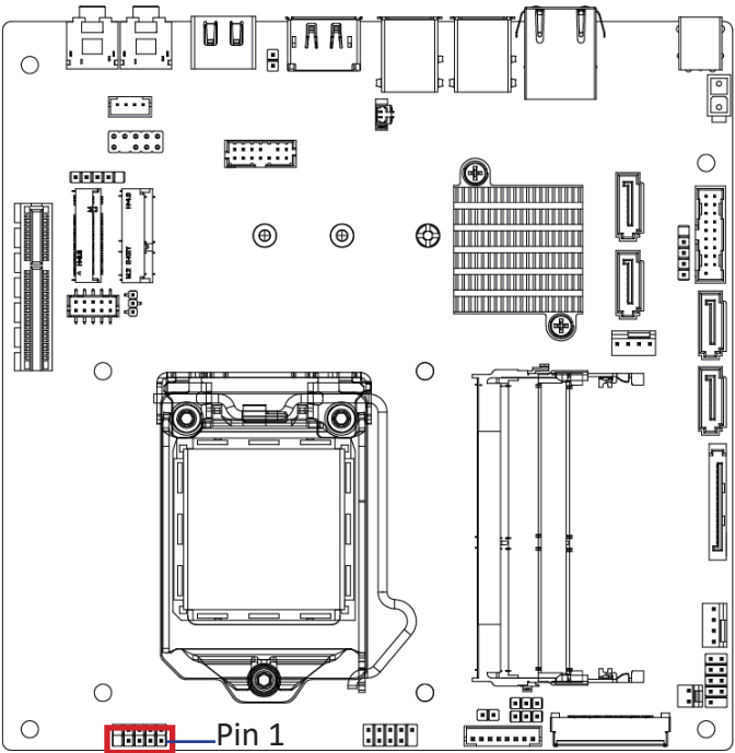
USB 2.0 Header
