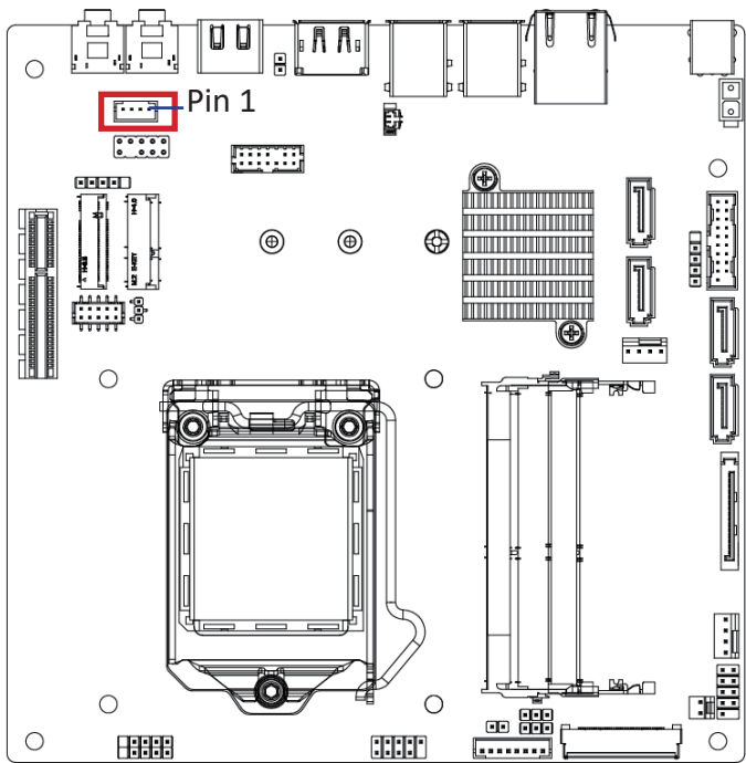
LCD_VCC Connector
