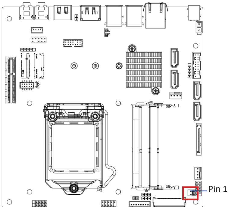
LCD_VCC Connector
