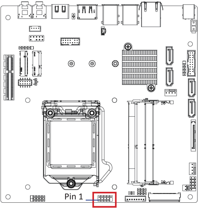
USB 2.0 Header
