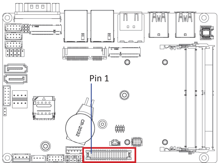
LVDS Connector
