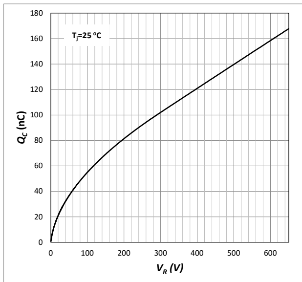
Fig. 7 Capacitive Charge
