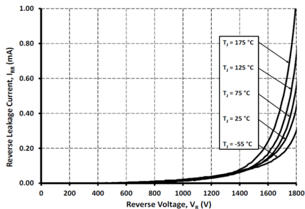
Reverse Characteristics vs. Junction Temperature
