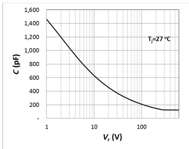
Capacitance Curve
