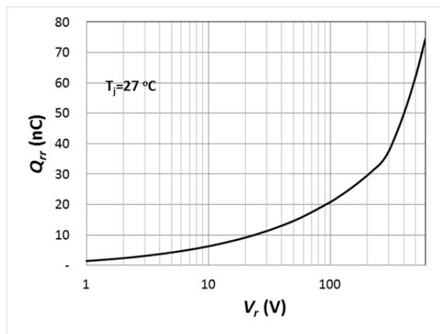
Recovery Charge
