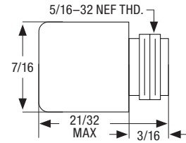
CYLINDRICAL LENS CAP
