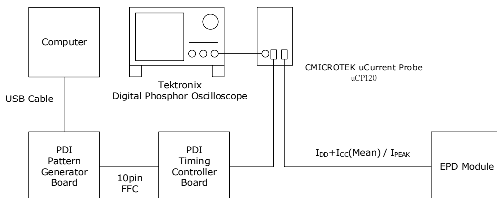
Figure 3-3 Current Measurement
