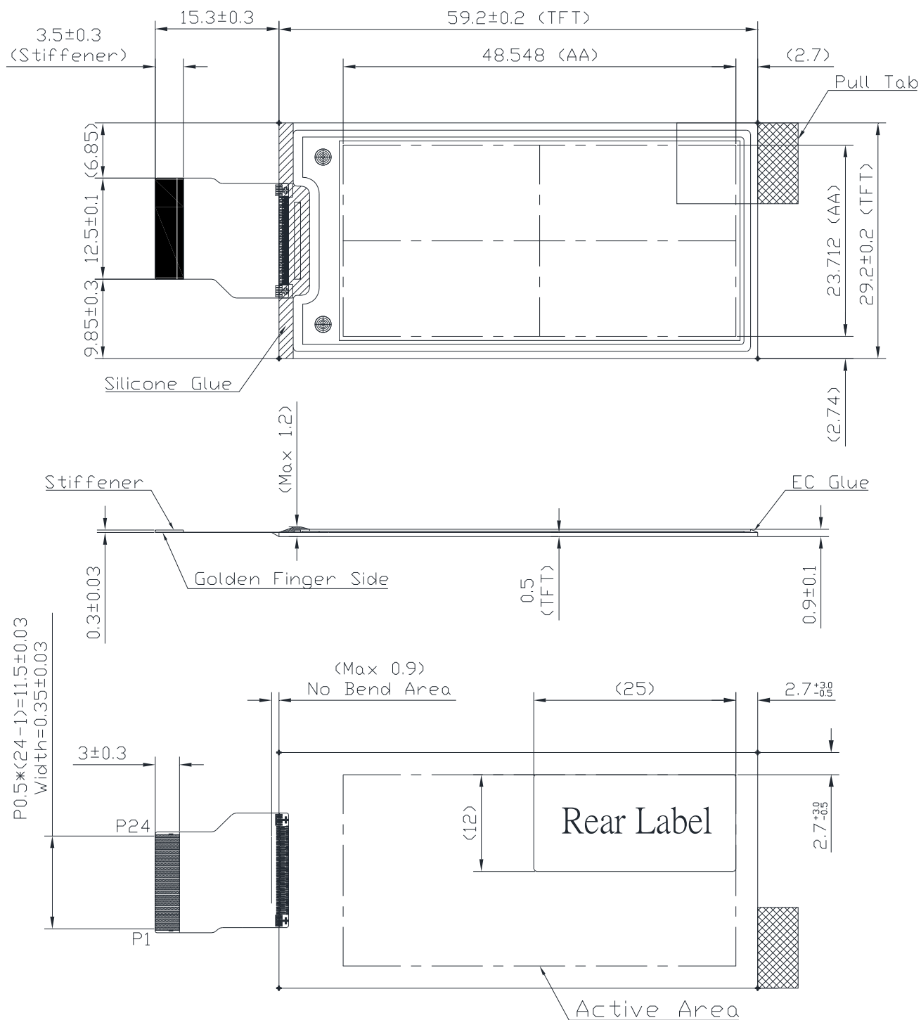
Figure 1-1 EPD Drawing
