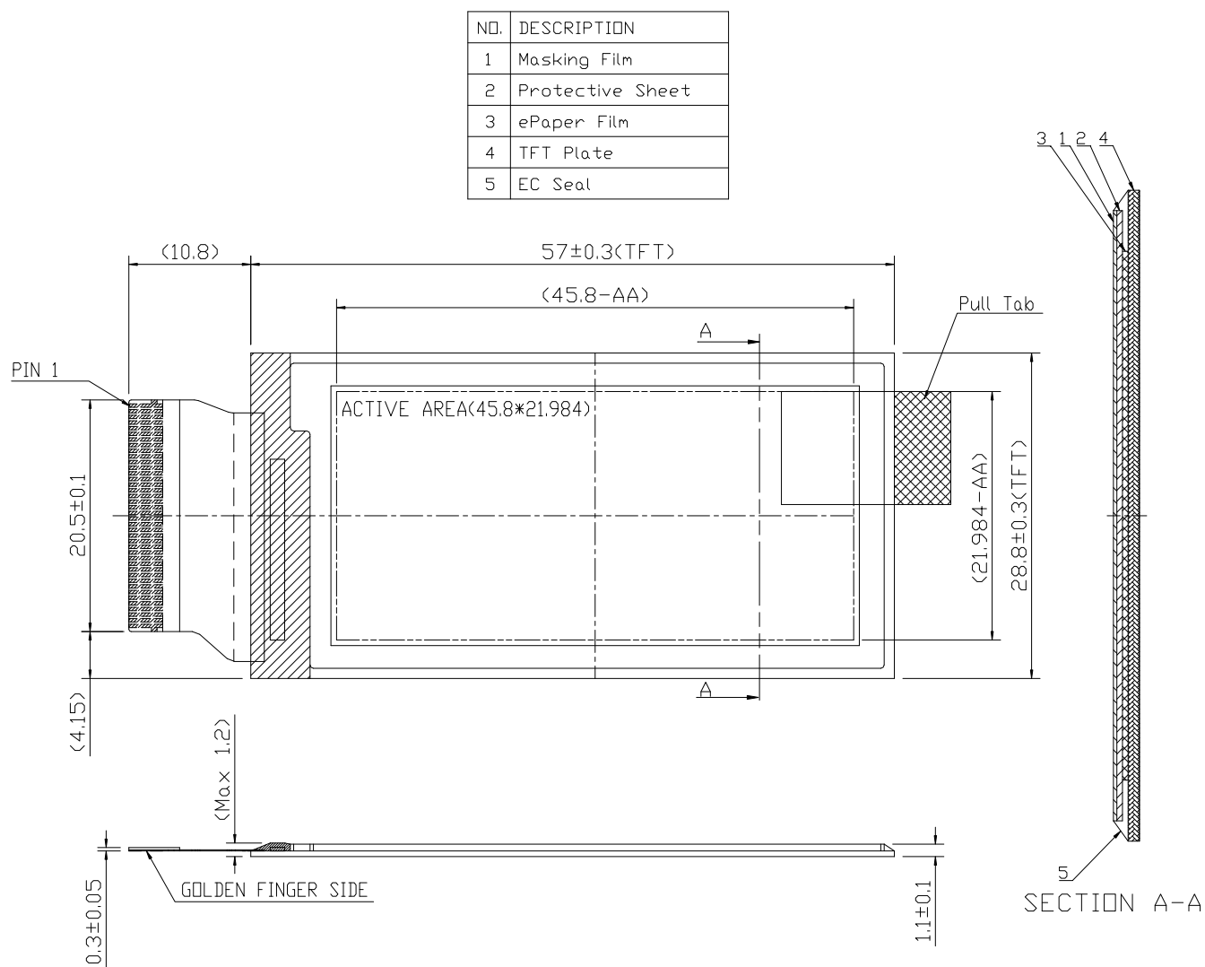
Figure 1-1 EPD Drawing
