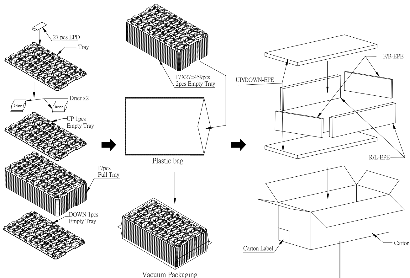
Figure 7-1 Packing Diagram
