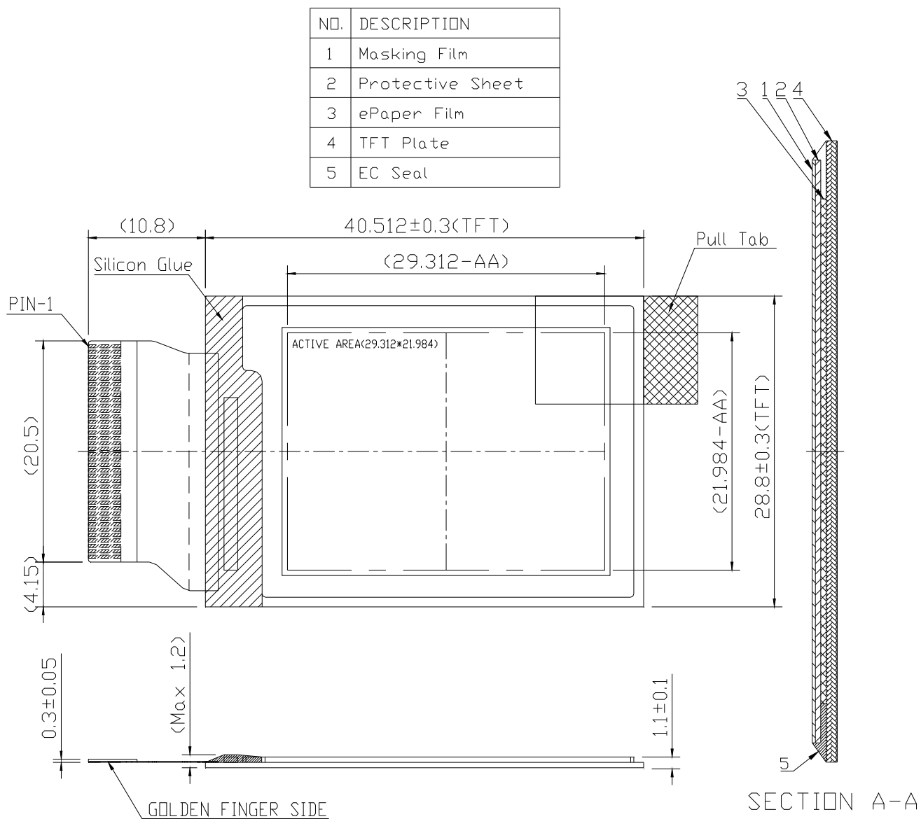
Figure 1-1 EPD Drawing
