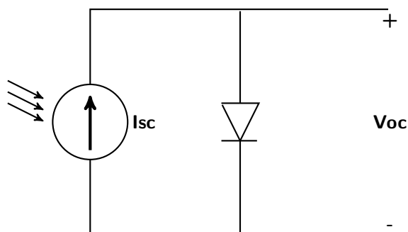
Figure 9: PV cell first order model
