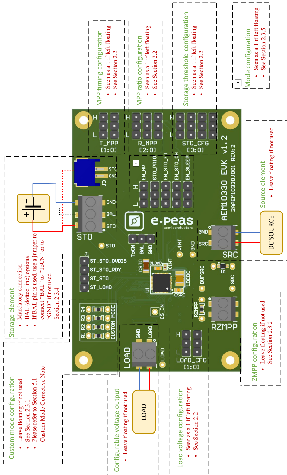
Figure 1: Connection Diagram
