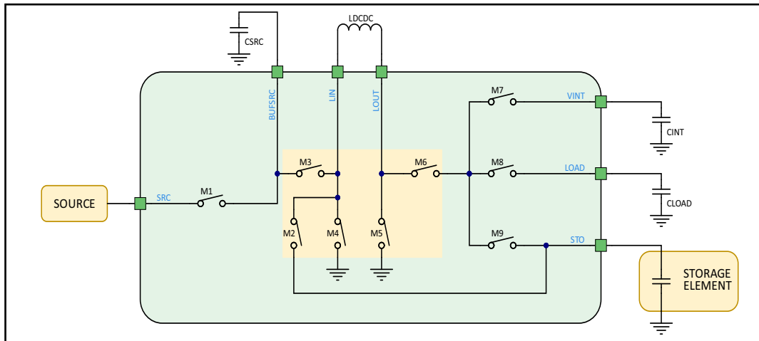
Figure 4: Simplified Schematic View of the AEM00330
