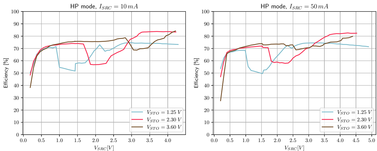
Figure 13: DCDC Efficiency from SRC to STO for 10 mA and 50 mA in High Power Mode
