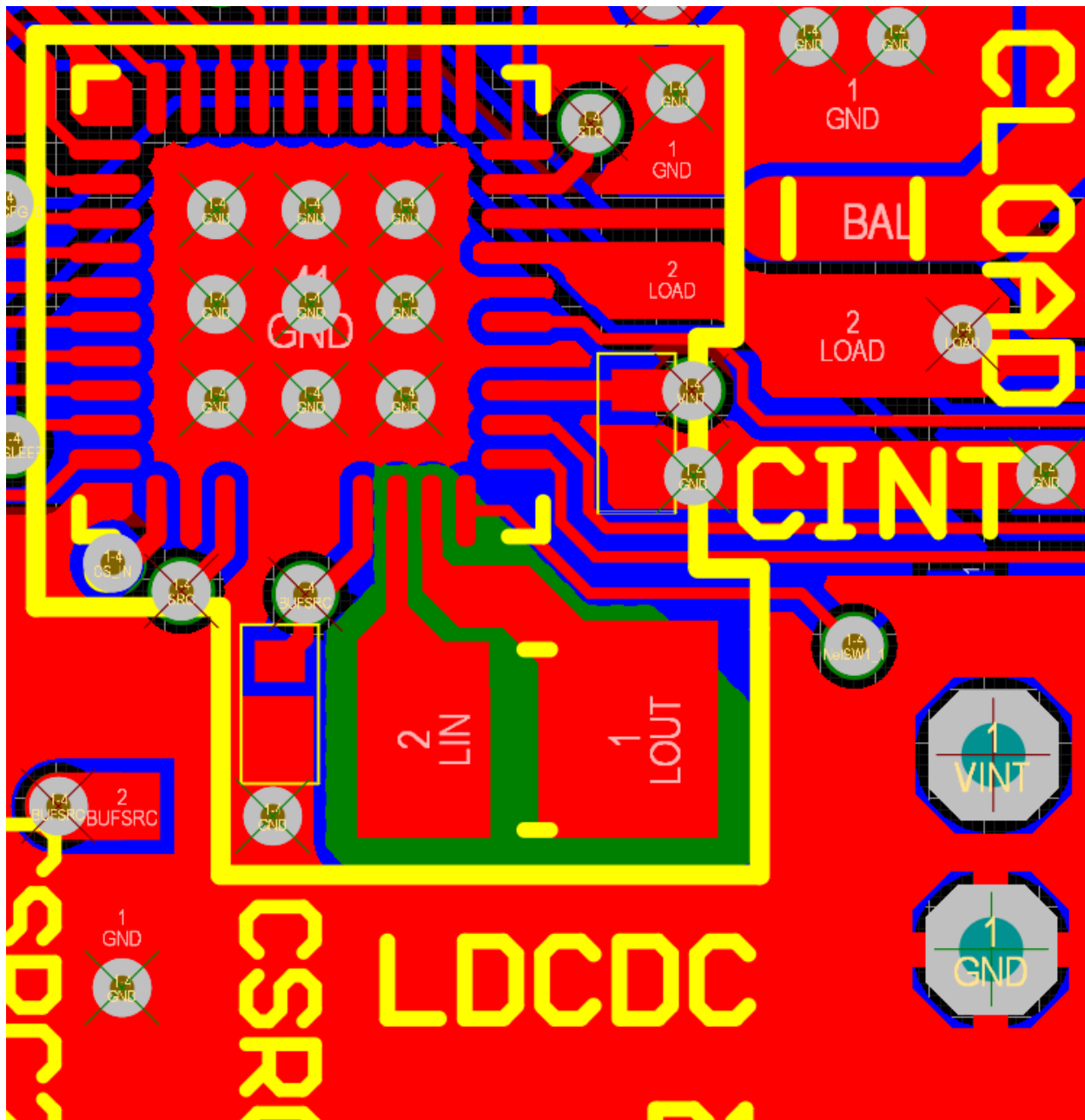
Figure 18: Layout Example for the AEM00330 and its Passive Components
