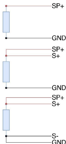
Resistance Thermometer
