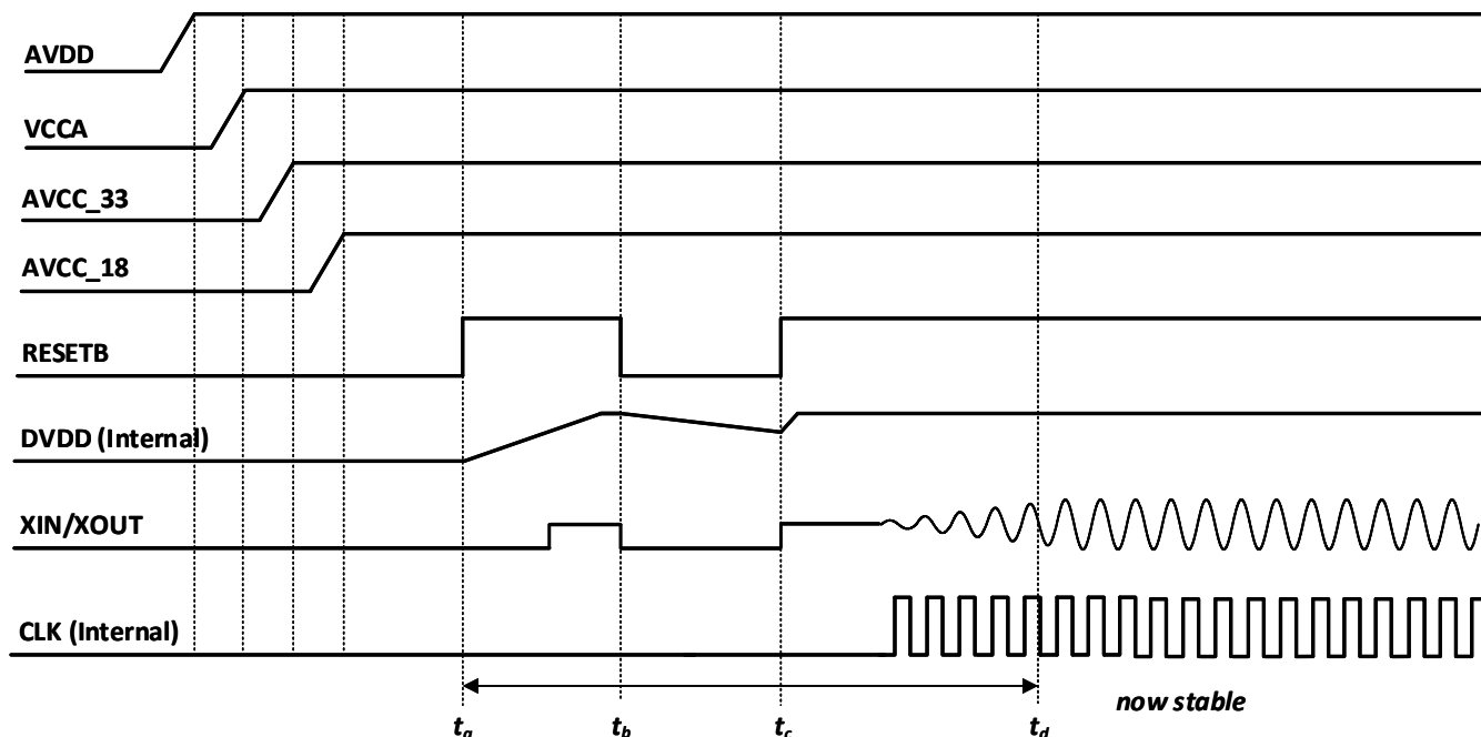
Figure 20 - Crystal with internal oscillator
