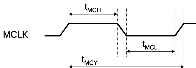
Figure 17 - Clock Timing Diagram
